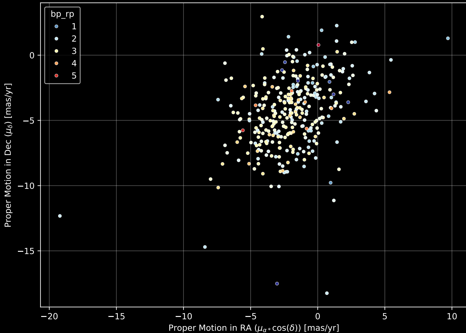
APOGEE DR17 Field: [350-04] Proper Motion Diagram (n= 328)
