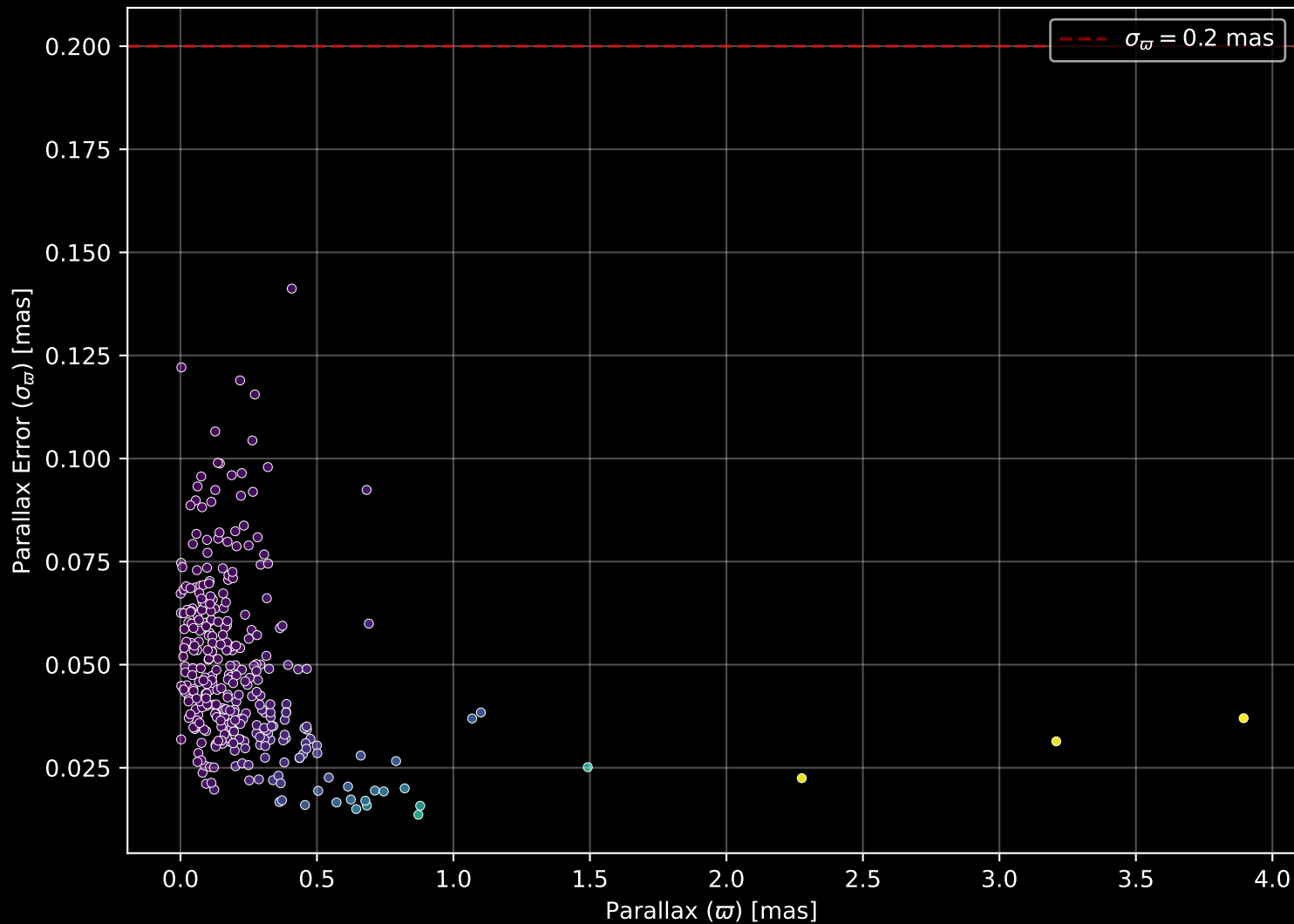
APOGEE DR17 Field: [350-04] Parallax Quality (n= 328)
