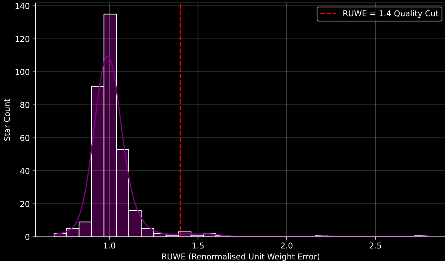
GAPOGEE DR17 Field [350-04] RUWE Distribution (n= 328)
