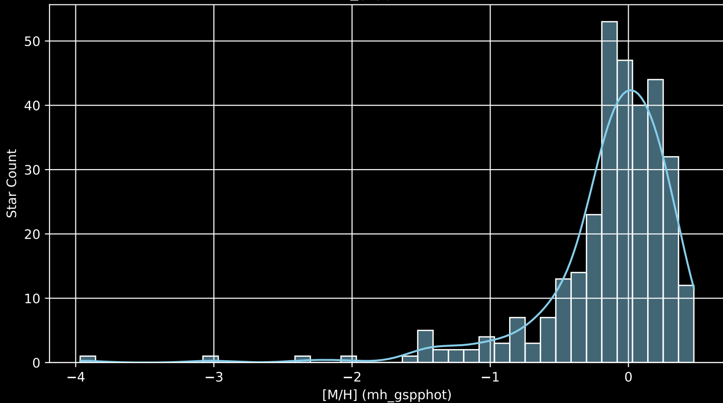
APOGEE DR17 Field: [350-04 [M/H] (mh_gspphot) (n= 318)
