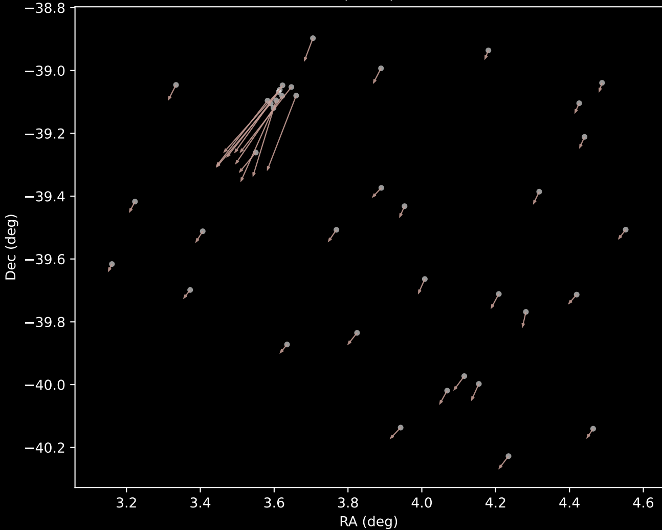
APOGEE DR17 Cluster 11 Proper Motion Vectors (n=39)
