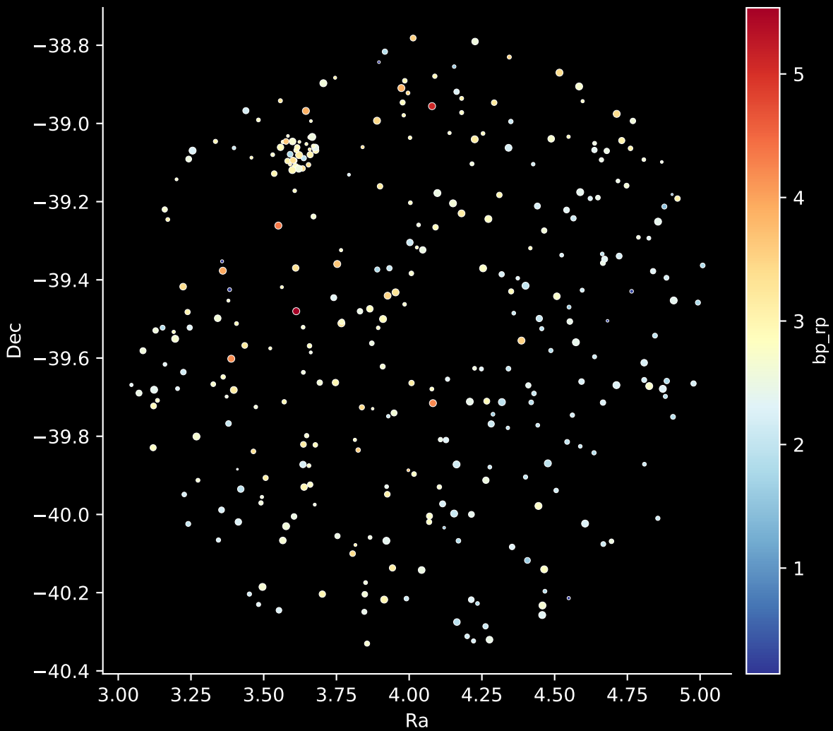
APOGEE DR17 Field: [350-04] Stars: 328
